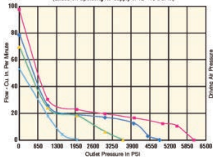
SM-3X-060 PUMP PERFORMANCE
