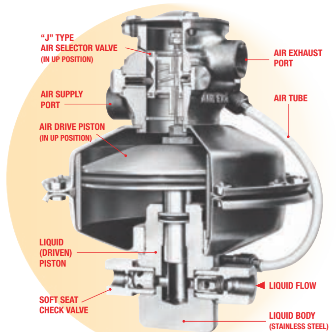
Pump Air Piston in UP Position
