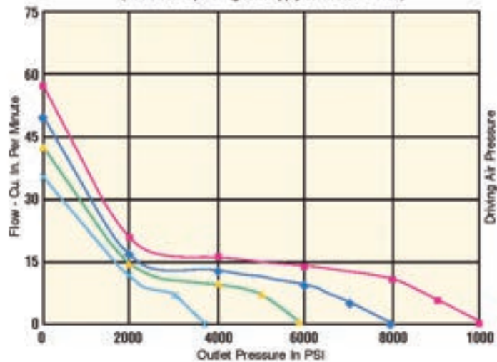
SM-3X-100 PUMP PERFORMANCE
