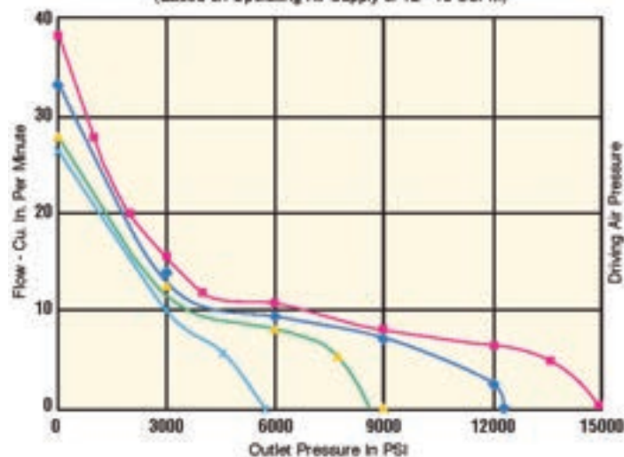
SM-3X-150 PUMP PERFORMANCE
