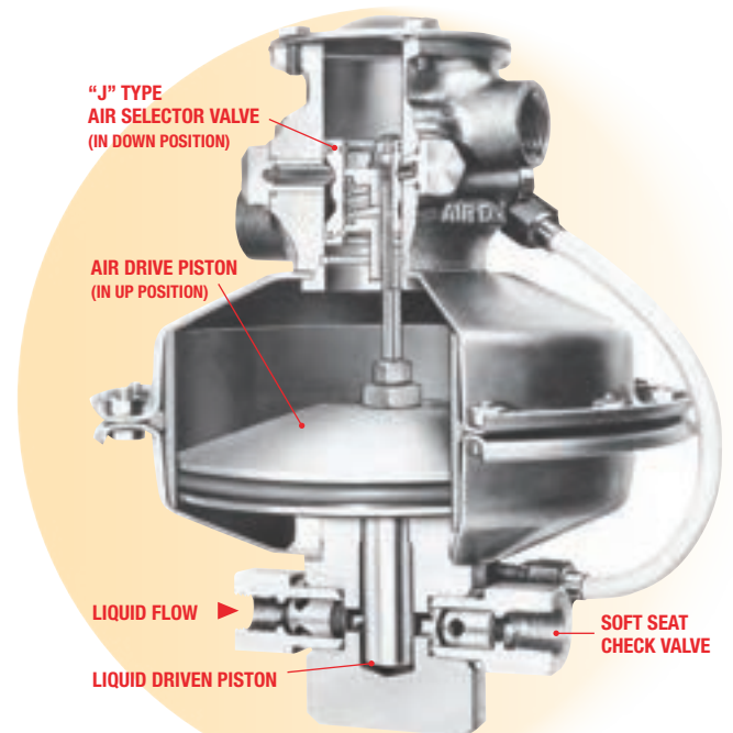
Pump Air Piston in DOWN Position
