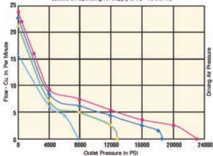
SM-3X-225 PUMP PERFORMANCE
