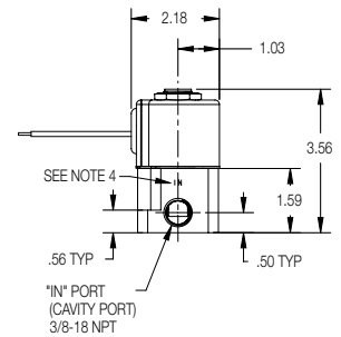
2-Way Normally Closed Grommet Housing
