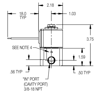
3-Way Line Connect Grommet Housing
