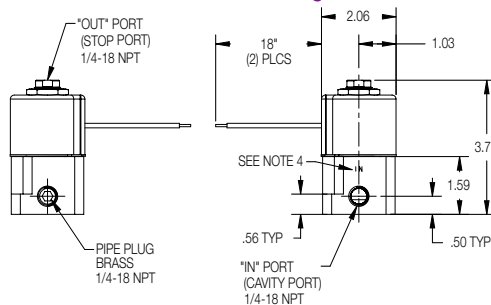
2-Way Normally Open Grommet Housing
