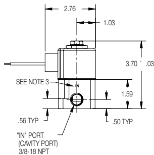
3-Way Line Connect Conduit Housing
