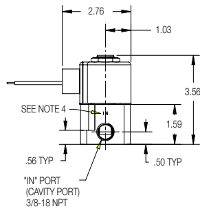
2-Way Normally Closed Conduit Housing
